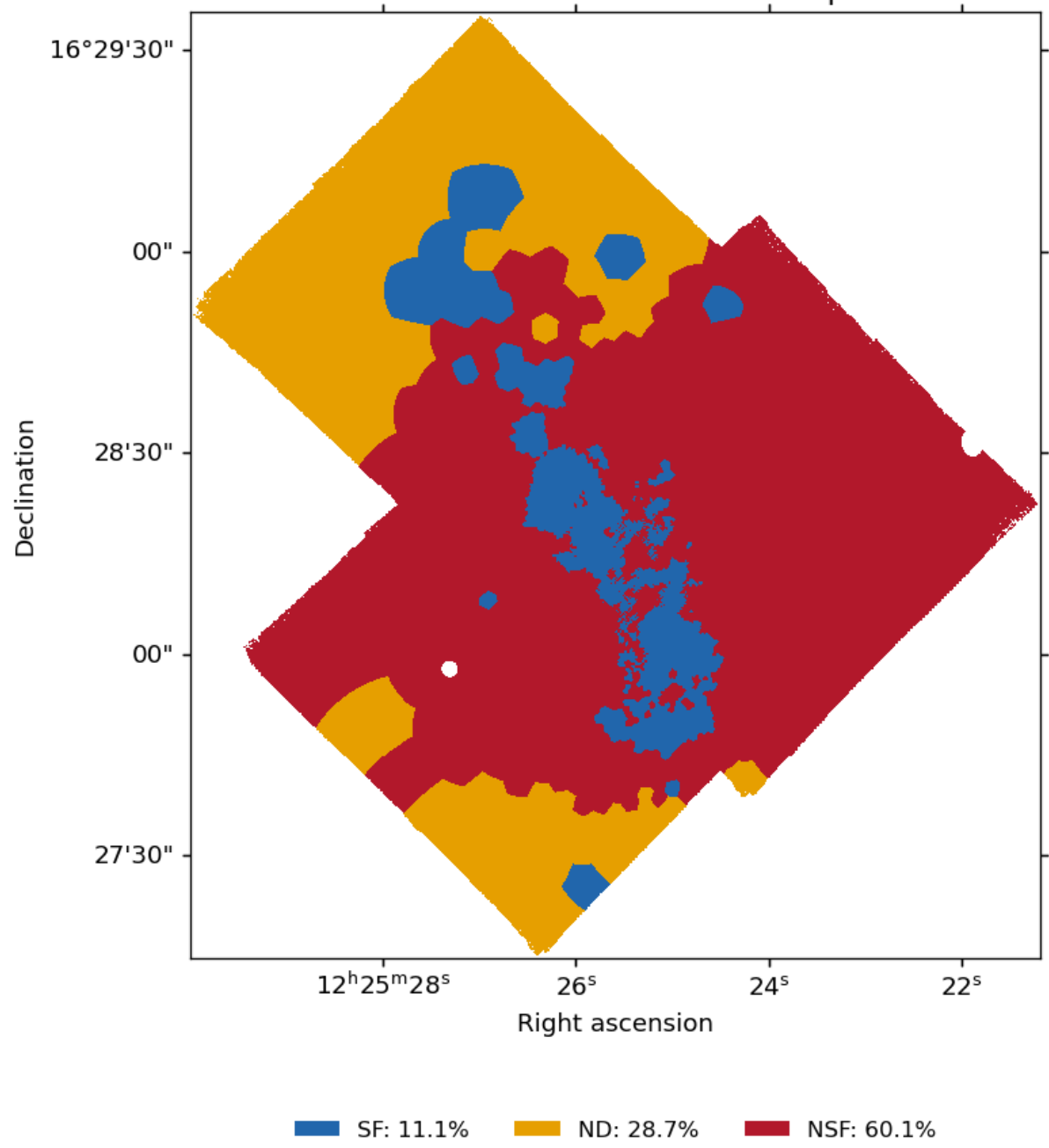
NGC4383 | pre-peak spatial categories White: outside the valid-disc footprint
