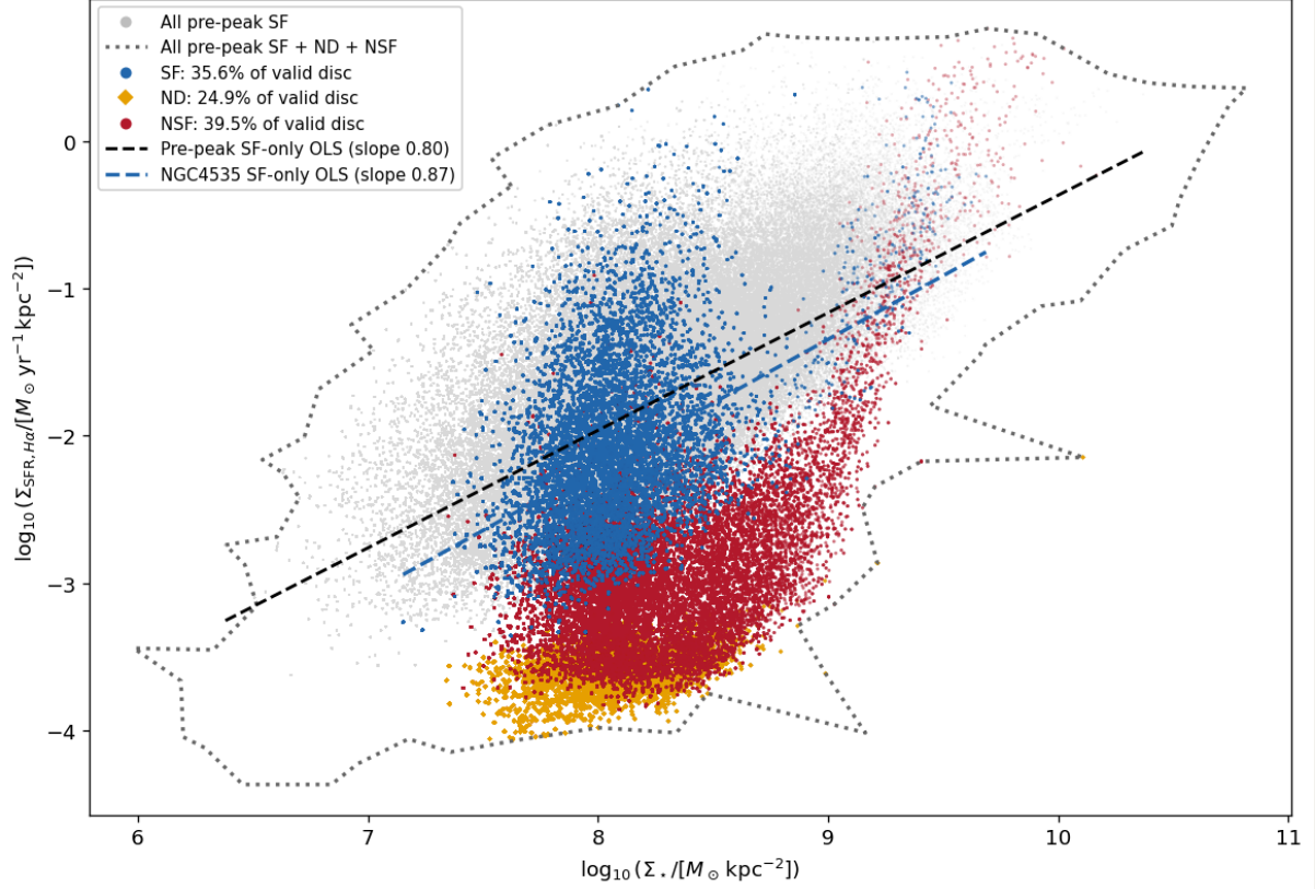
NGC4535 | pre-peak Plotted SF / ND / NSF = 187,113 / 130,687 / 207,301
