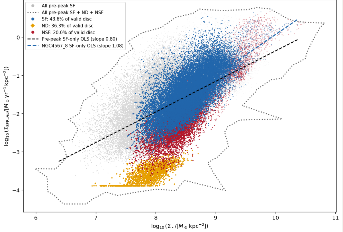
NGC4567_8 | pre-peak Plotted SF / ND / NSF = 222,533 / 185,310 / 102,275
