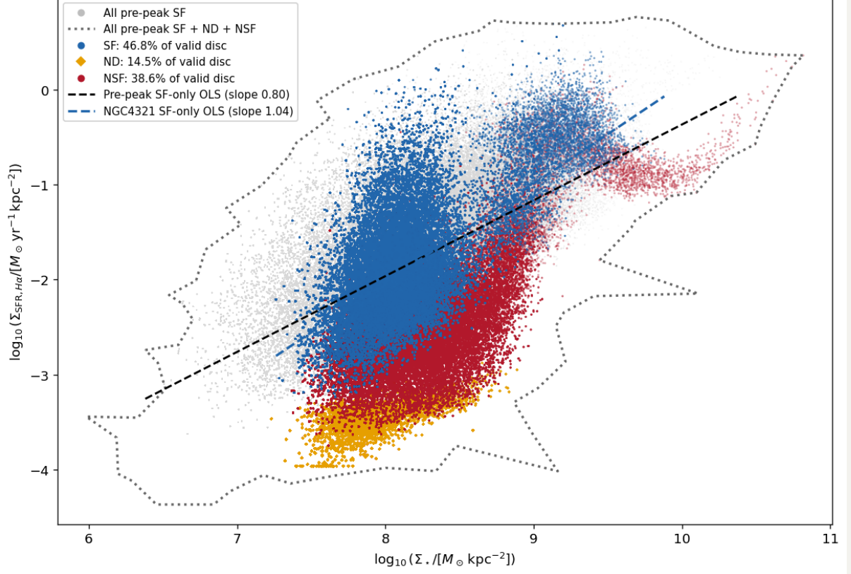
NGC4321 | pre-peak Plotted SF / ND / NSF = 454,131 / 141,086 / 374,942
