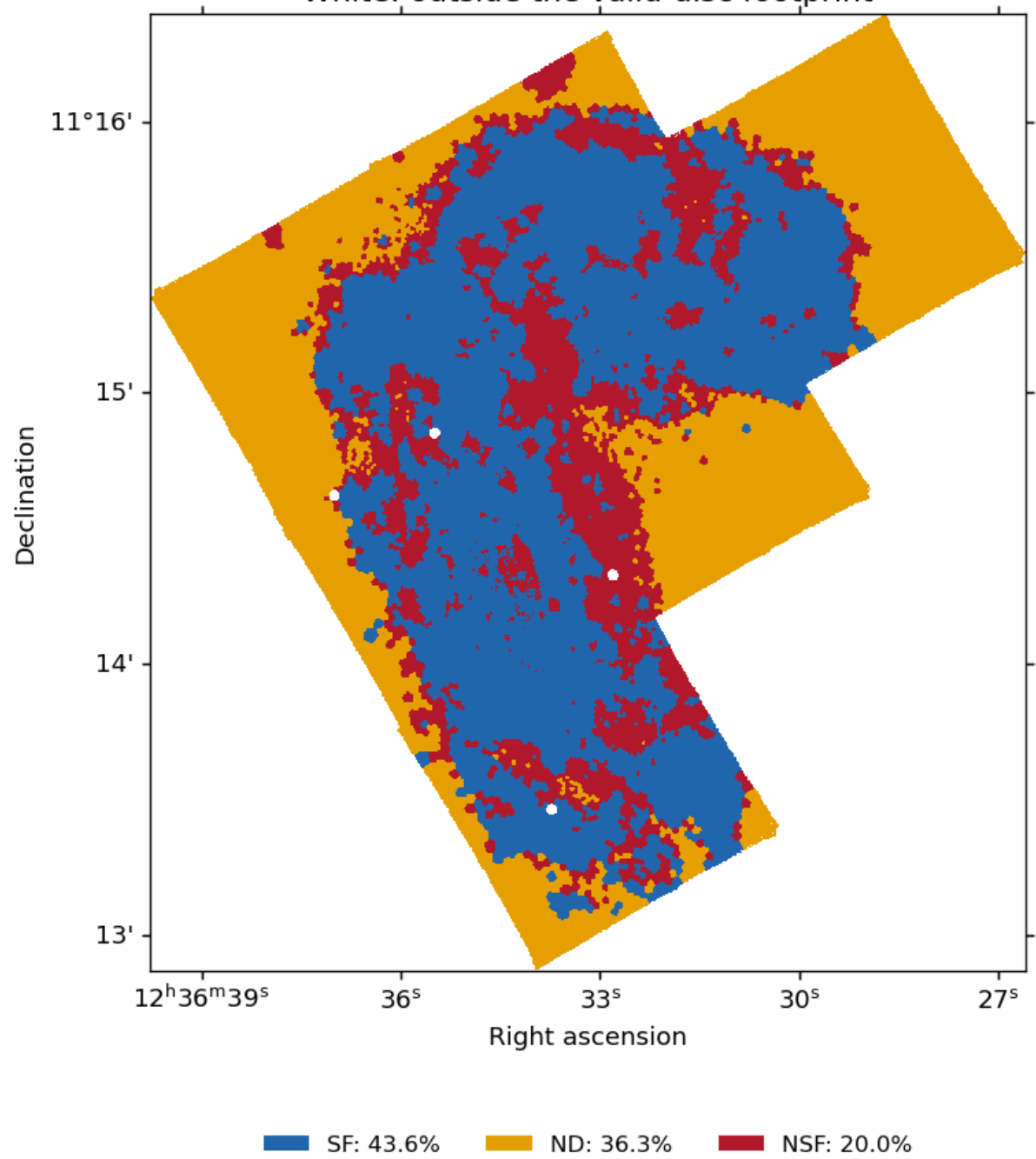
NGC4567_8 | pre-peak spatial categories White: outside the valid-disc footprint
