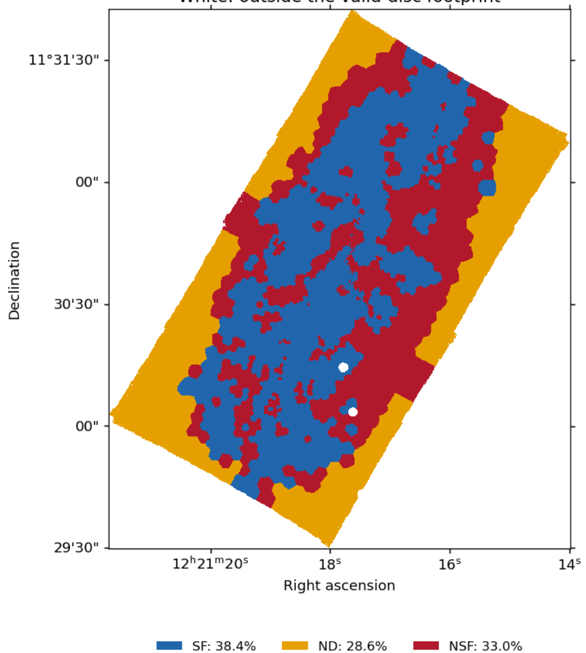
NGC4294 | pre-peak spatial categories White: outside the valid-disc footprint
