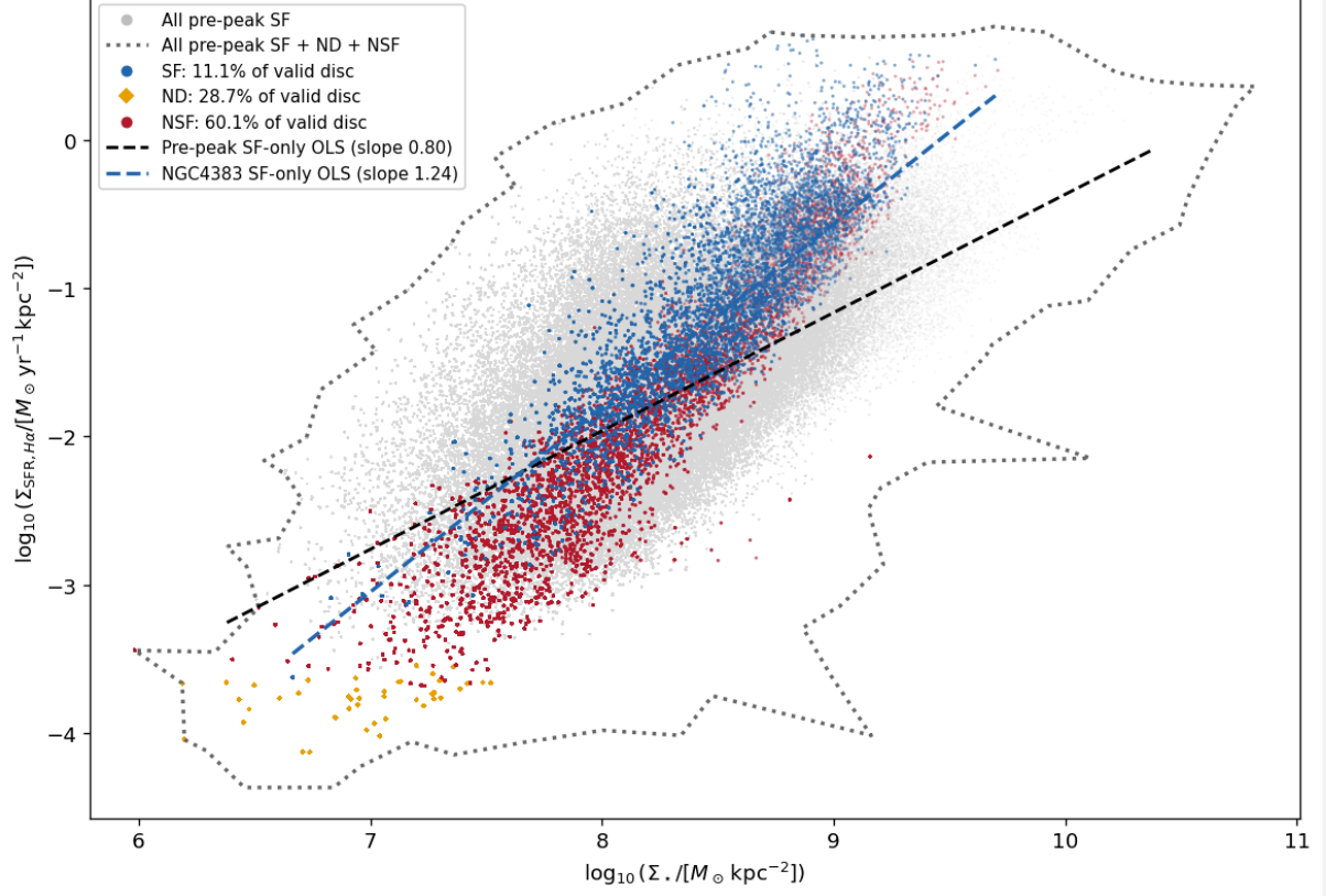
NGC4383 | pre-peak Plotted SF / ND / NSF = 25,212 / 65,261 / 136,558
