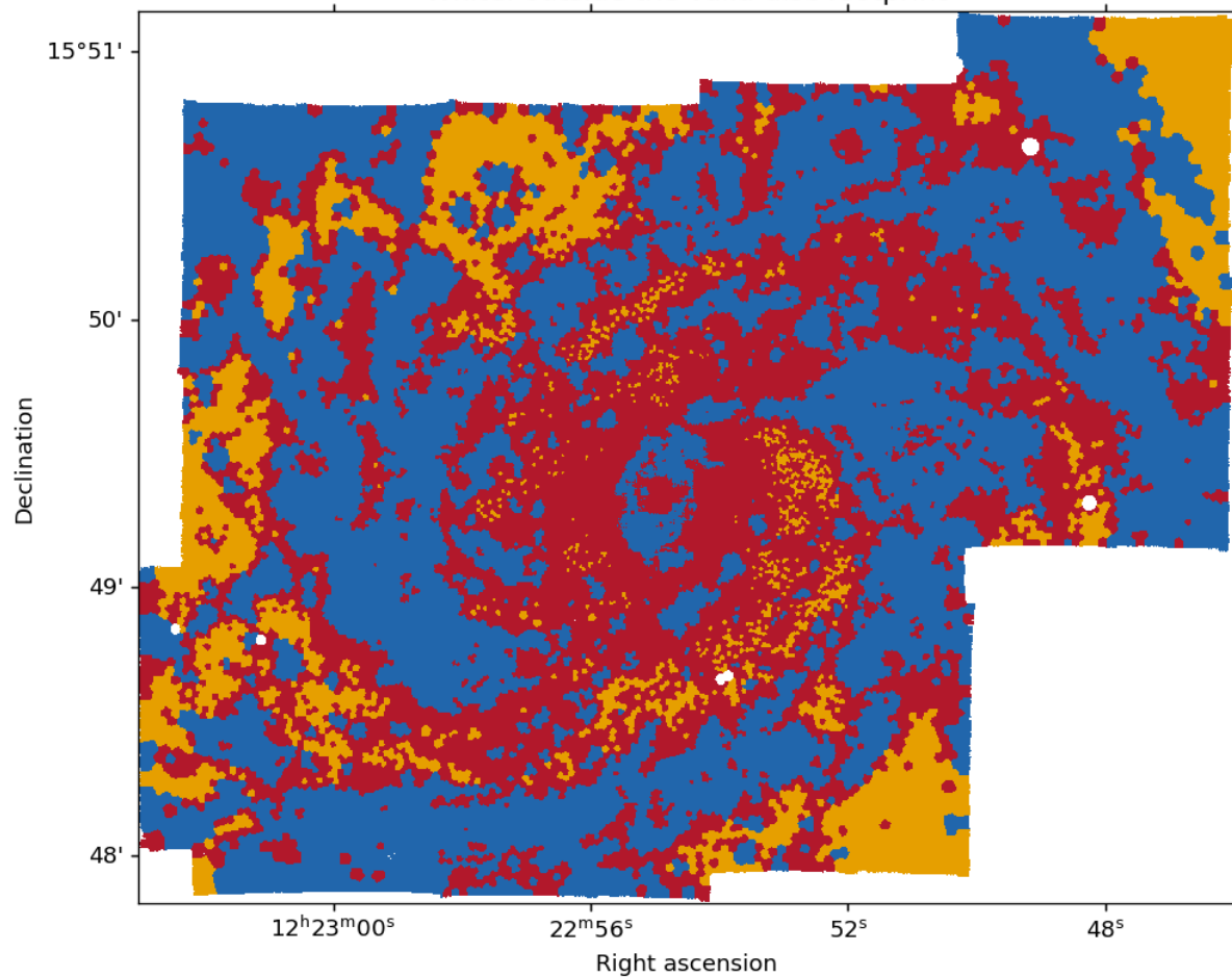
NGC4321 | pre-peak spatial categories White: outside the valid-disc footprint
