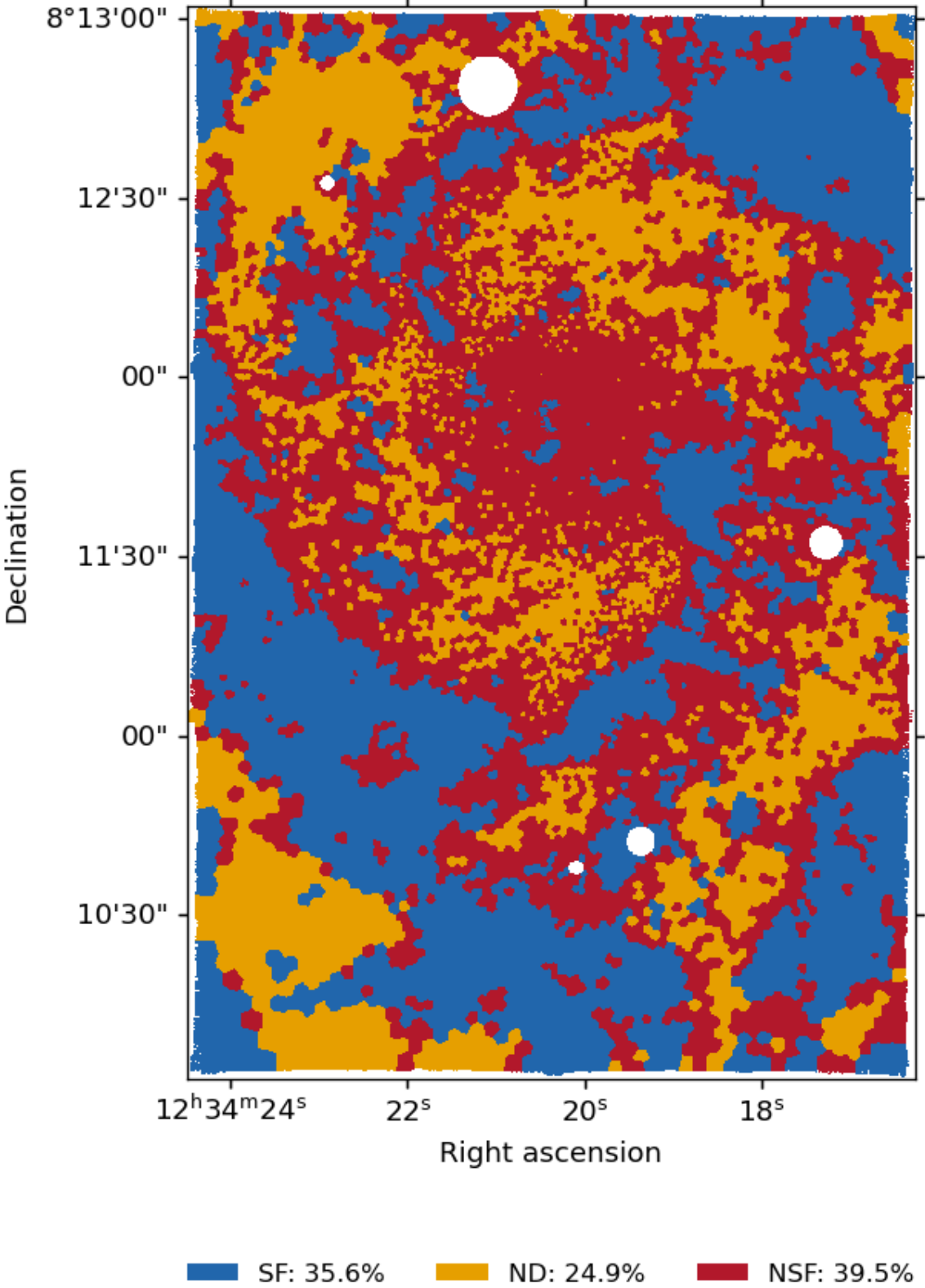
NGC4535 | pre-peak spatial categories White: outside the valid-disc footprint
