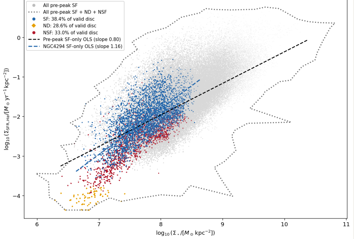
NGC4294 | pre-peak Plotted SF / ND / NSF = 68,833 / 51,275 / 59,247
